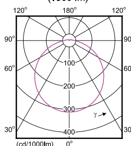
Polar intensity diagram (1300 lm)
