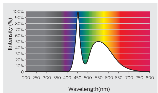
Spectrum high lumen LEDbulb 6500K
