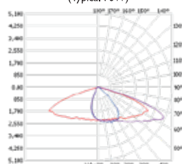
Polar Candela Distribution (Typical 70W)
