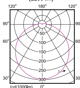
Polar intensity diagram (2200 lm)
